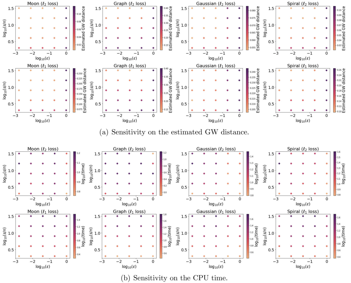
Figure 4. Impact of the subsample size s and the regularization parameter \epsilon for Spar-GW on the GW distance estimation (panel (a)) and computational time (panel (b)). The mean over 10 runs are reported.
