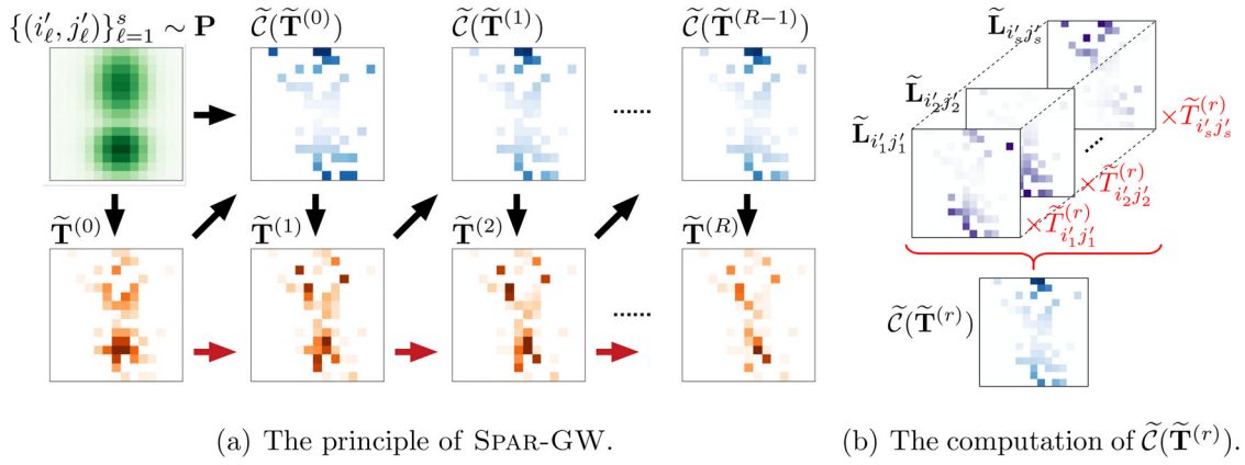
Figure 1. (a) An illustration of our Spar-GW. The nonzero elements of each matrix are labeled with colors. The arrows between \tilde{T}^{(r)} 's are applied when using the proximal gradient algorithm. (b) An illustration of the computation of \tilde{C}(\tilde{T}^{(r)}) in the r th iteration.
